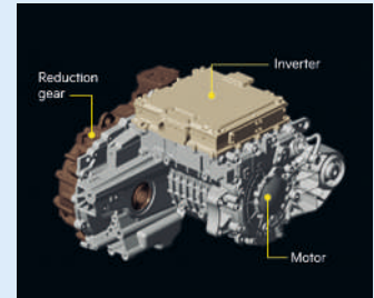
Rear Motor
