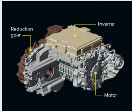
Rear Motor
