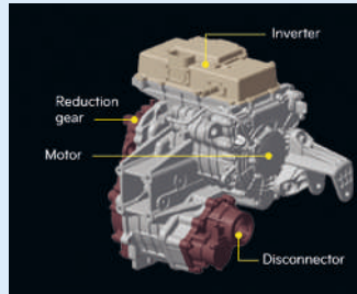
Front Motor
